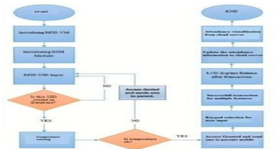
Fig. 11. FLOWCHART
