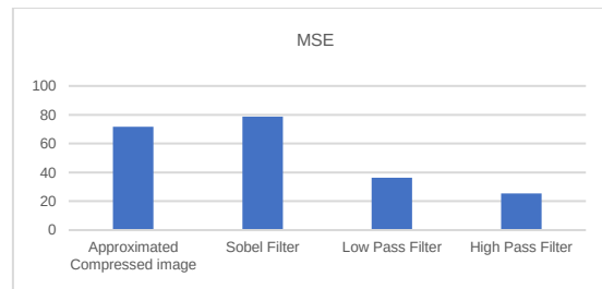
Fig 5.2: Representation Of Mse Values Of Approximated Compressed Image, Sobel Filter, Low Pass Filter, High Pass Filter
