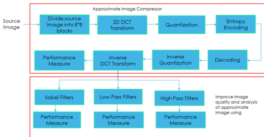
Fig 1: Block Diagram For Proposed System
