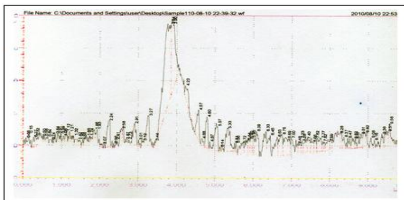
Figure 6: RP-HPLC Chromatogram of thermal degradation
