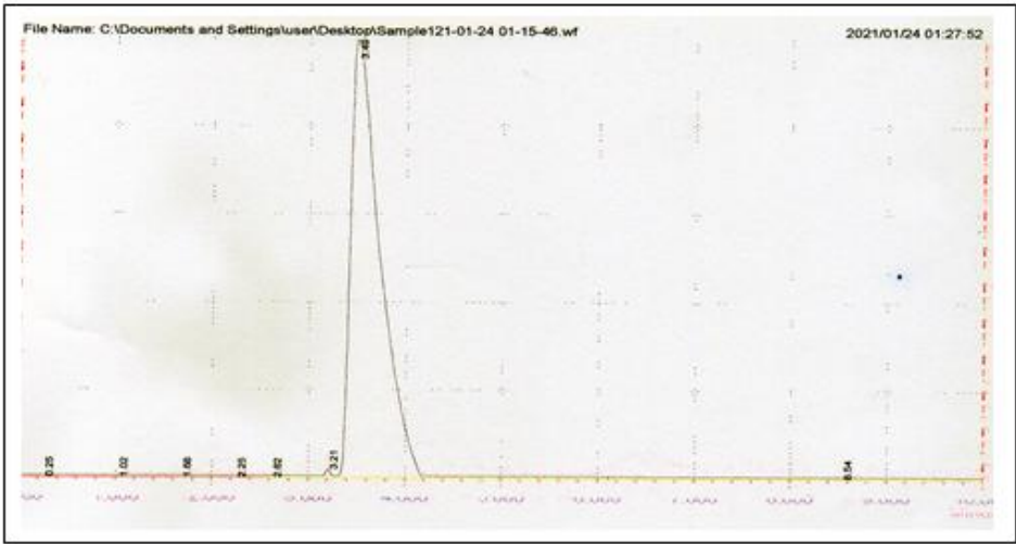
Figure 10: RP- HPLC Chromatogram obtained after method optimization
