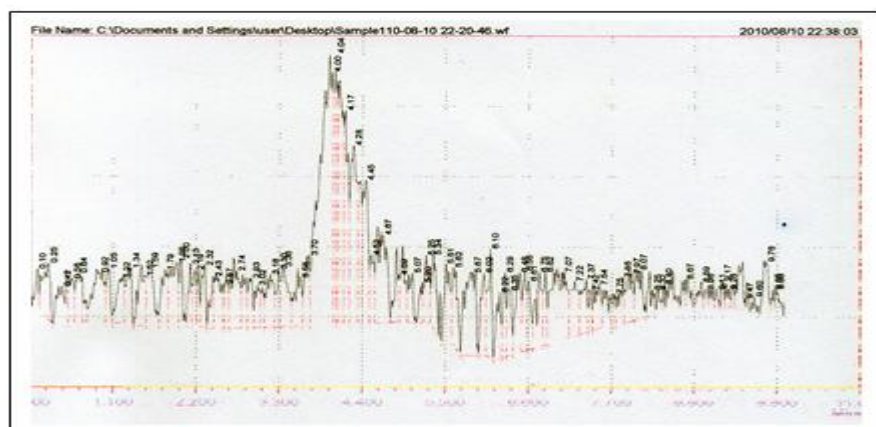
Figure 5: Photolytic degradation RPHPLC Chromatogram
