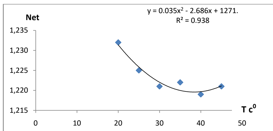
Fig (3): The distribute Net count with change temperature for Cs-137 total area
