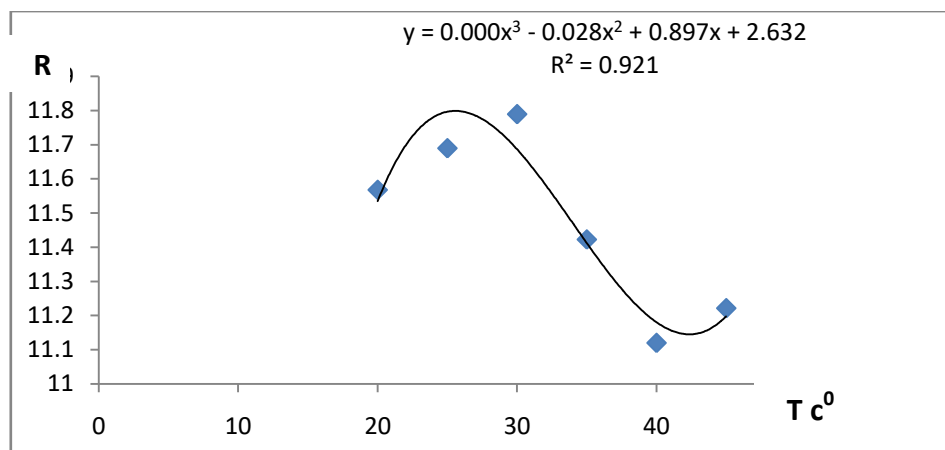
Fig (9): The distribute the energy resolution with change temperature for(Cs-137) photo peak.
